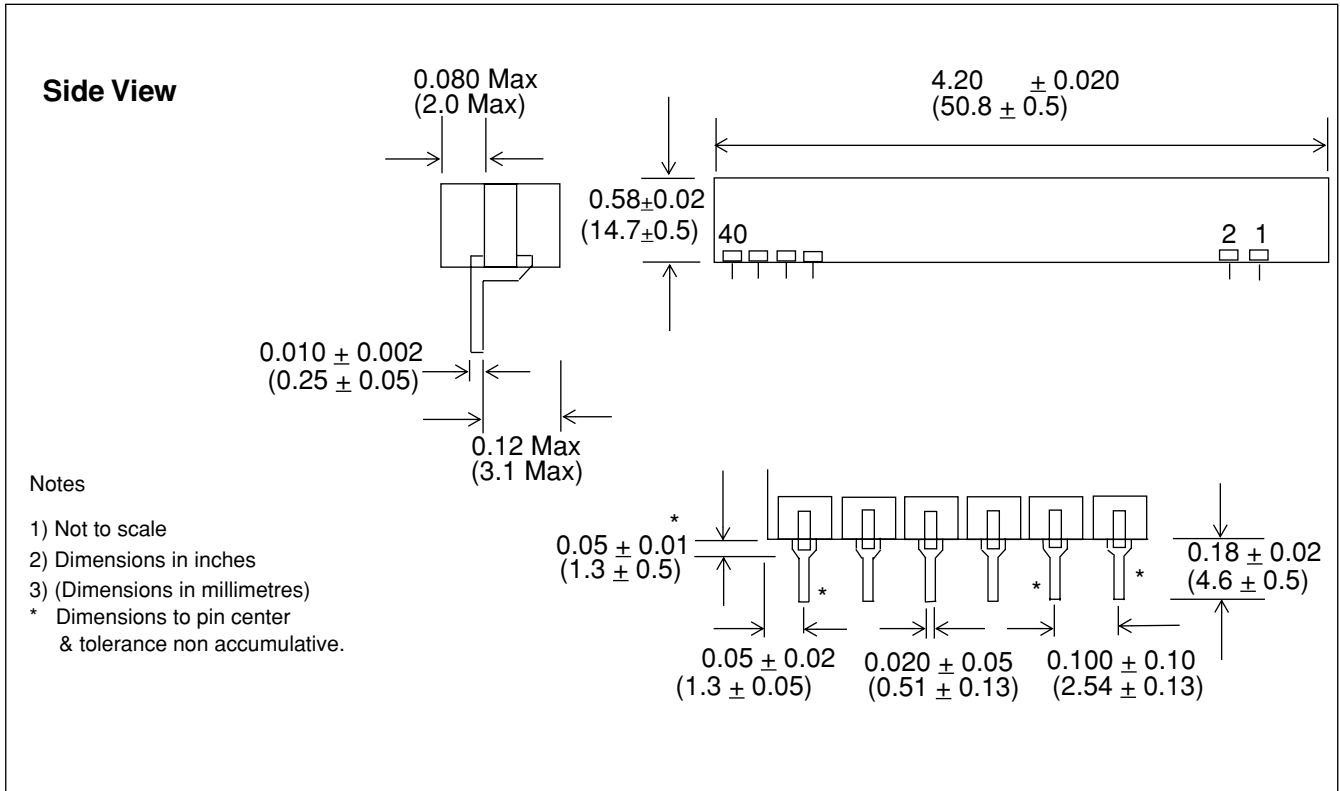
Figure 10 - Mechanical Data
