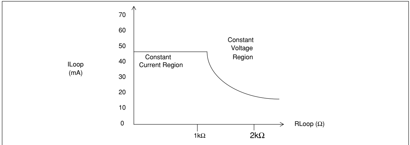
Graph 1 - Iloop/Rloop Characteristics
