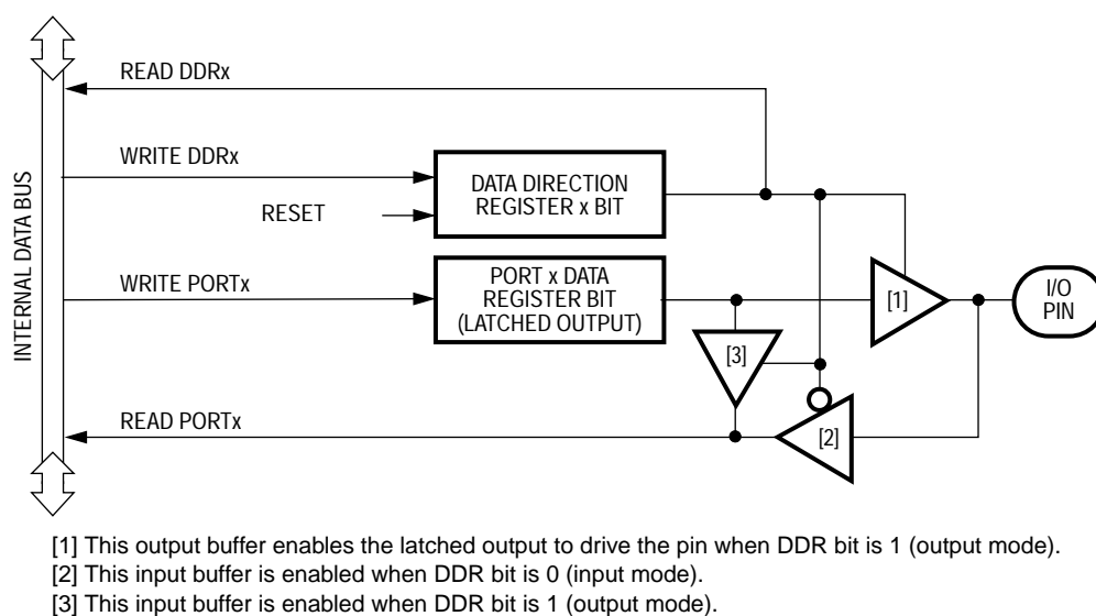
Figure 7-2. I/O Circuitry
