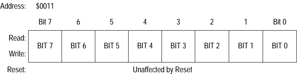
Figure 9-4. SCI Data Register (SCDR)
