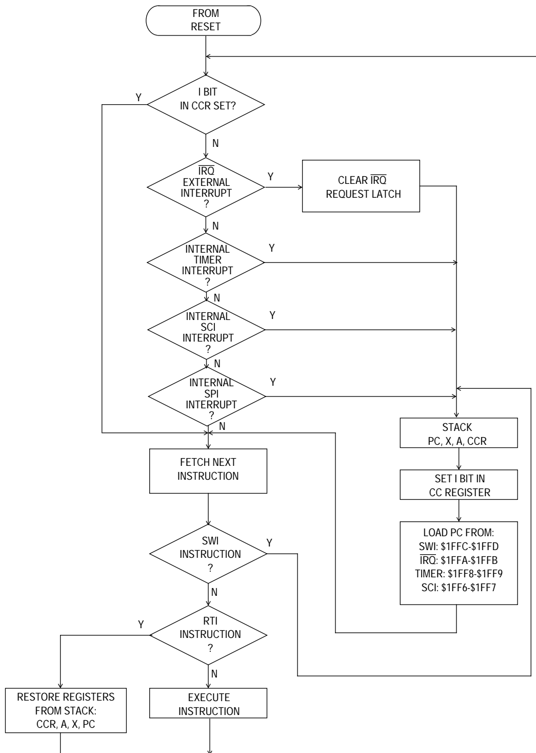
Figure 4-1. Interrupt Flowchart
