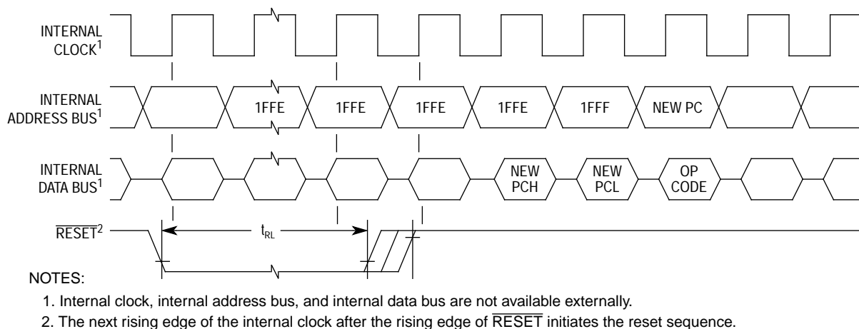
Figure 13-6. External Reset Timing
