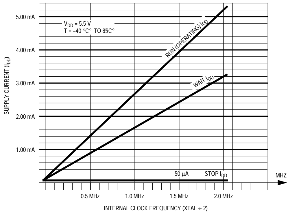
Figure 13-2. Maximum Supply Current Versus Internal Clock Frequency, V_{DD} = 5.5 V
