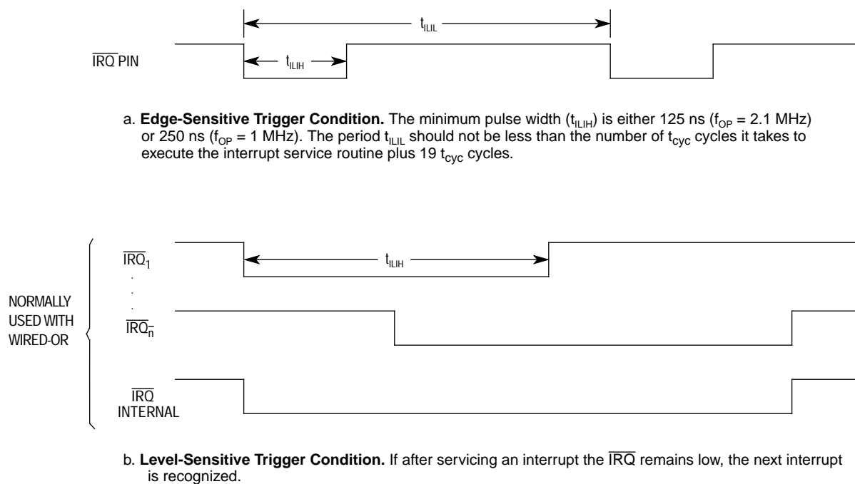
Figure 13-5. External Interrupt Timing
