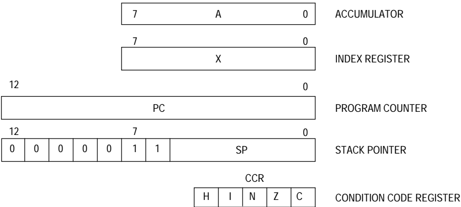
Figure 3-1. Programming Model
