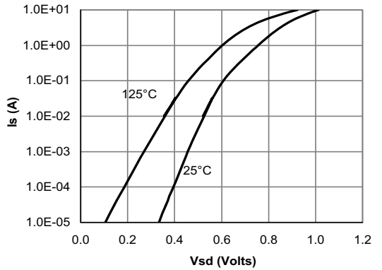
Figure 6: Body-Diode Characteristics
