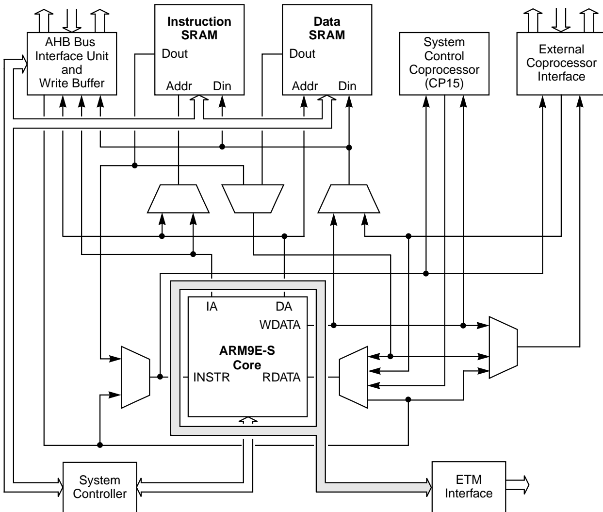
Figure 1 CW001102 Block Diagram
