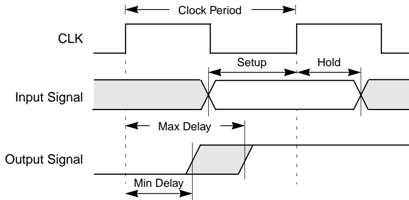
Figure 2 AC Specifications
