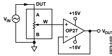
Figure 29. Test Circuit for Gain vs. Frequency
