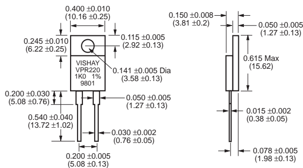
FIGURE 1 - VPR220 DIMENSIONS
