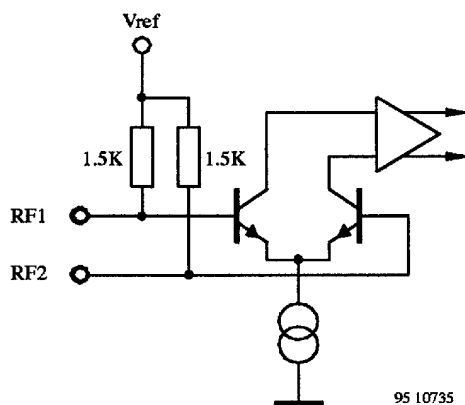
Figure 7. RF input
