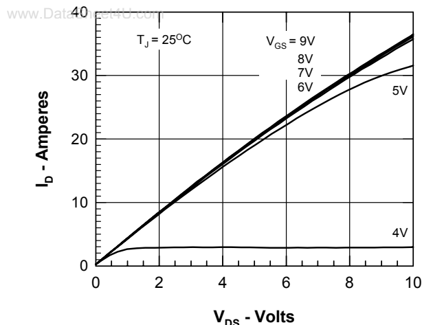
Figure 1. Output Characteristics at 25°C
