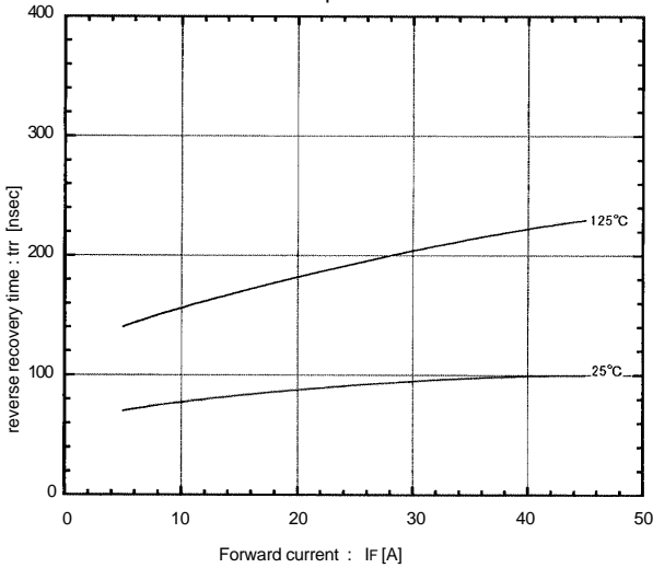
Reverse recovery time vs. Forward current -di/dt=90A / μsec
