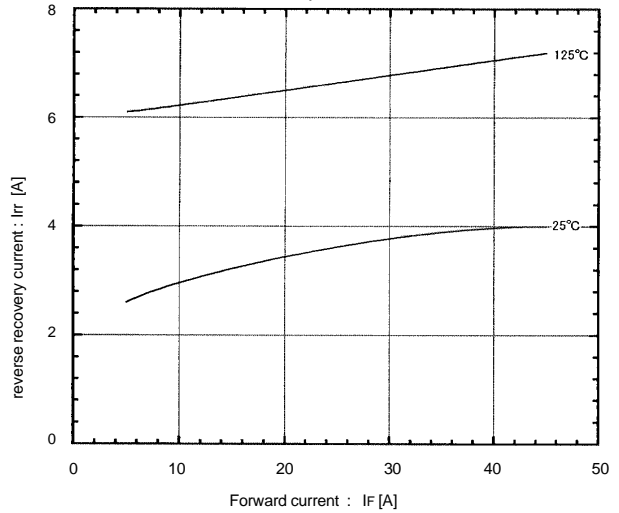
Reverse recovery current vs. Forward current -di/dt=90A / μsec
