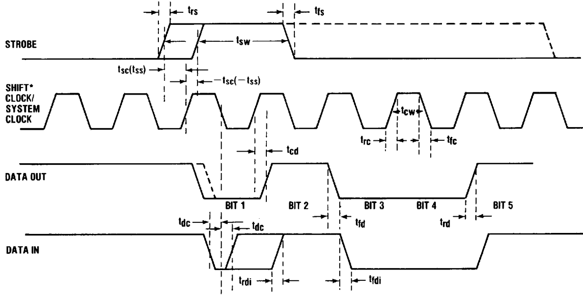
Figure 2C. Waveform Details
