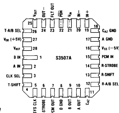
Pin Configuration—S3507A 28-Lead Chip Carrier
