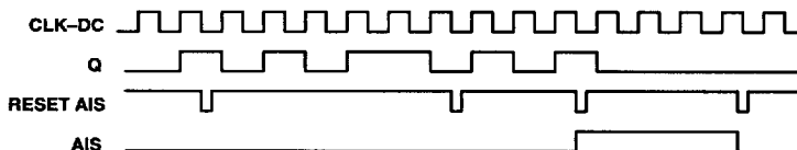
AIS WAVEFORMS
