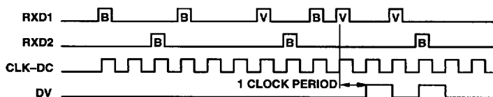
HDB3 DOUBLE VIOLATION WAVEFORMS
