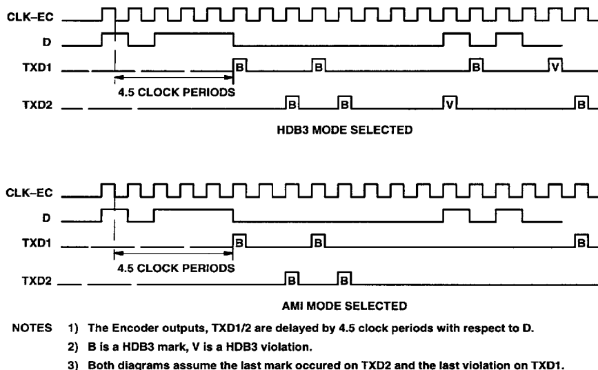
Fig. 3 HDB3/AMI Encoder waveforms
