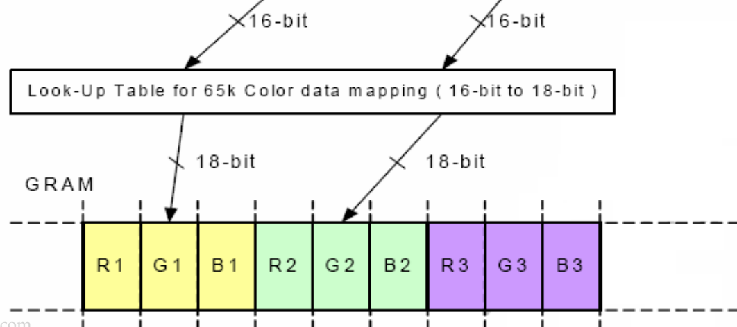
Figure 5.4.2 8-bit Data Bus GRAM Write/Read Data Format (65K)
