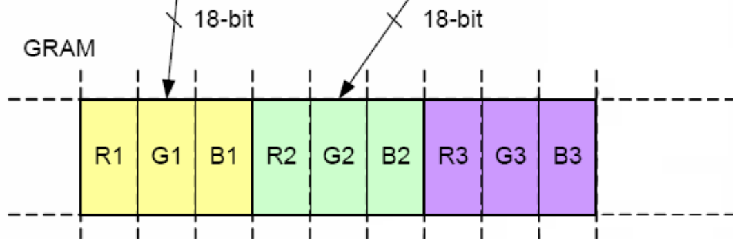
Figure 5.4.1 8-bit Data Bus GRAM Write/Read Data Format(262K)
