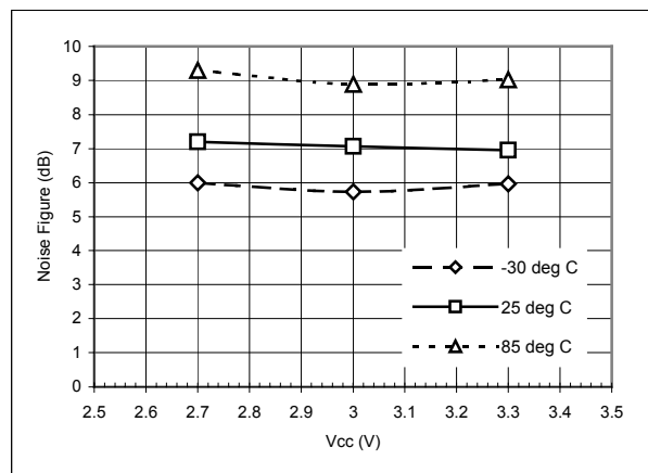
Figure 40. AMPS VGA+I/Q Noise Figure ( V_c = 2.5 V) at 85.38 MHz
