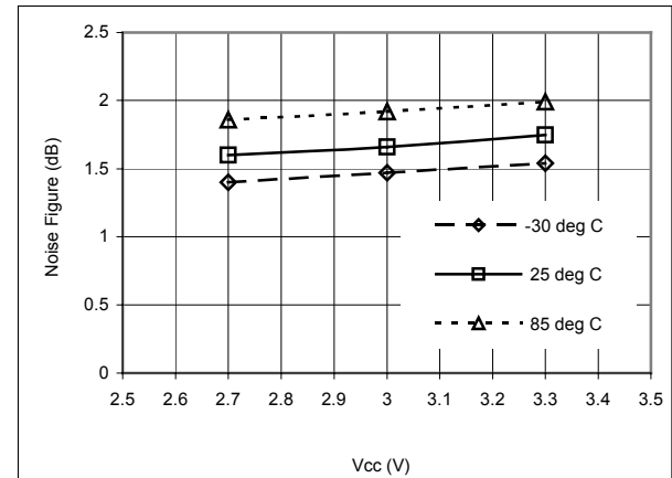
Figure 10. Cell CDMA LNA NF at 881 MHz
