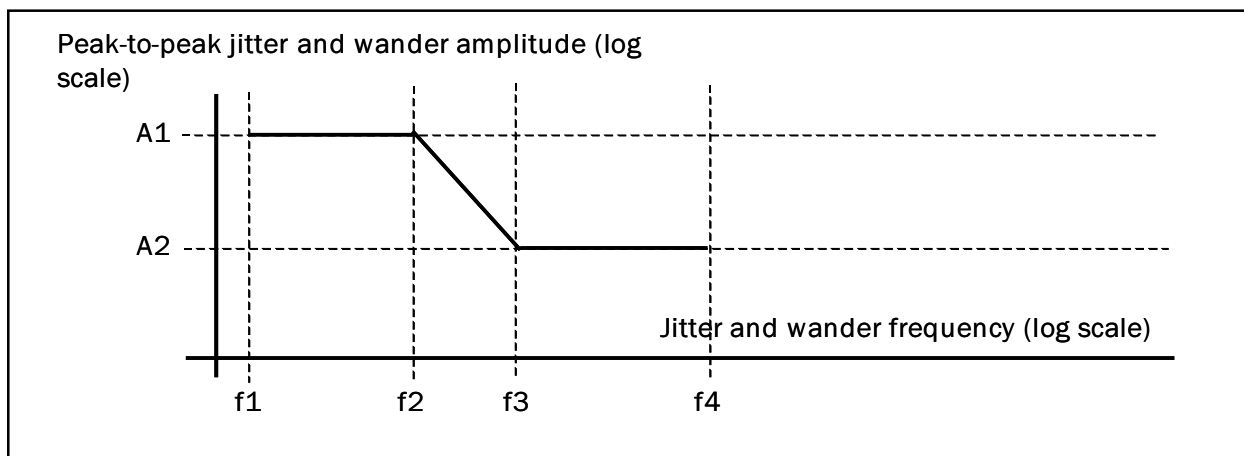
Figure 4. Minimum Input Jitter Tolerance (DS1/E1) (for inputs supporting G.783 compliant sources)
