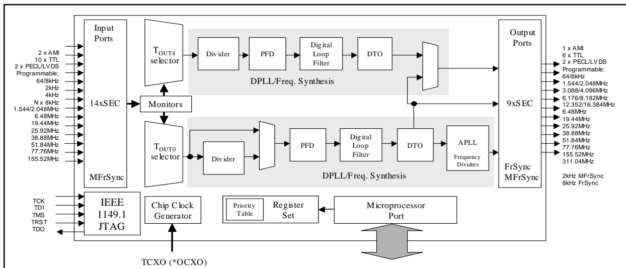
Figure 1. Simple Block Diagram
