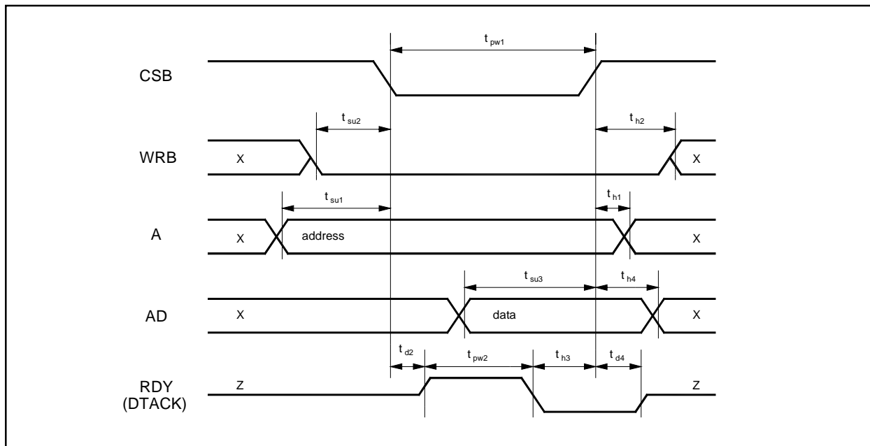
Figure 20. Write Access Timing in MOTOROLA Mode
