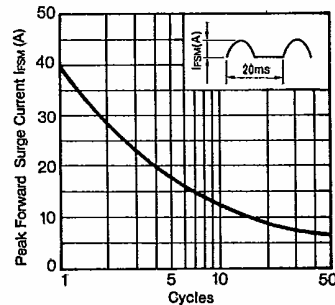
I_{FSM} Characteristics
