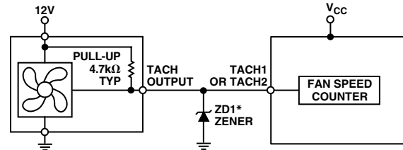
Figure 9b. Fan with Tach. Pull-Up to Voltage >6.5\text{ V} (e.g., 12 V) Clamped with Zener Diode
