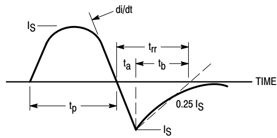
Figure 16. Diode Reverse Recovery Waveform
