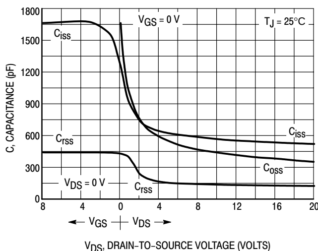
Figure 9. Capacitance Variation
