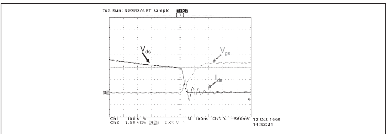
Figure 6: MDmesh™ Turn-on
