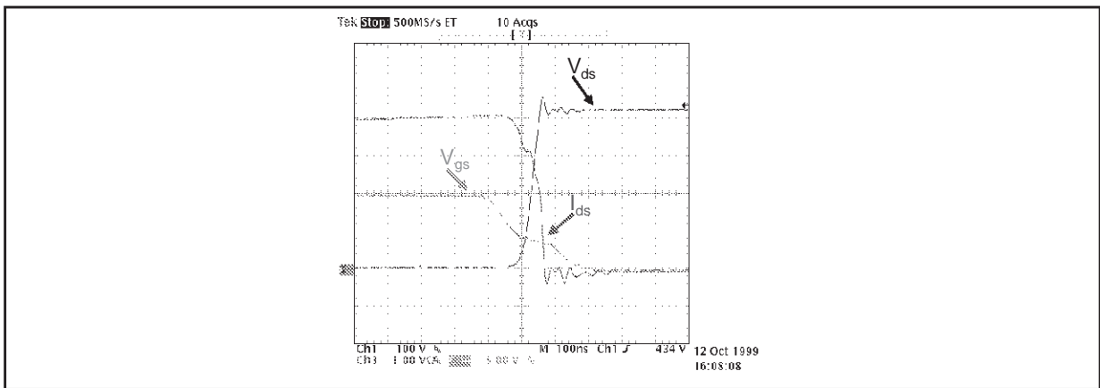
Figure 5: STW15NB50 Turn-off
