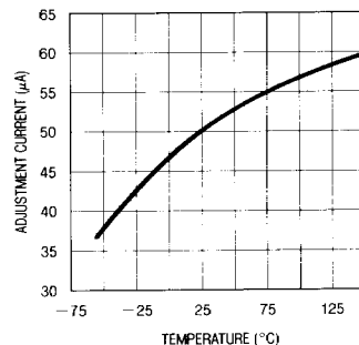
Adjustment Current
