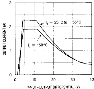
Current Limit (T0-3 and T0-220 Package)
