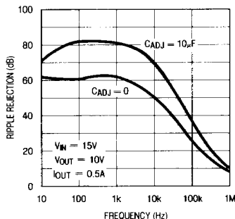
Ripple Rejection (dB)
