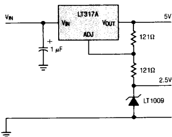
Regulator with Reference
