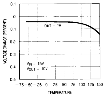
Load Regulation
