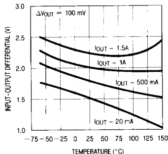
Dropout Voltage
