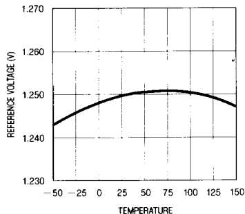
Temperature Stability
