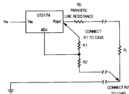
Connections for Best Load Regulation
