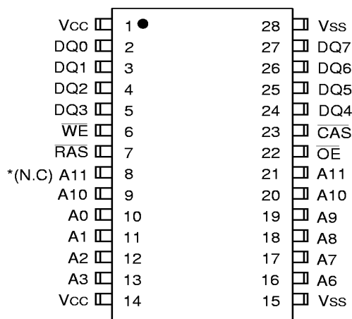
28Pin Plastic TSOP-II (300mil)
