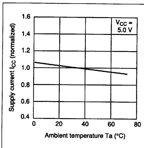
Supply Current vs. Ambient Temperature (1)
