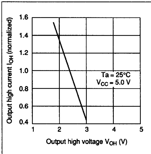
Output High Current vs. Output High Voltage
