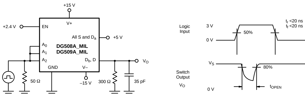
FIGURE 4. Break-Before-Make Interval
