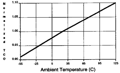
NORMALIZED TCO vs. TEMPERATURE
