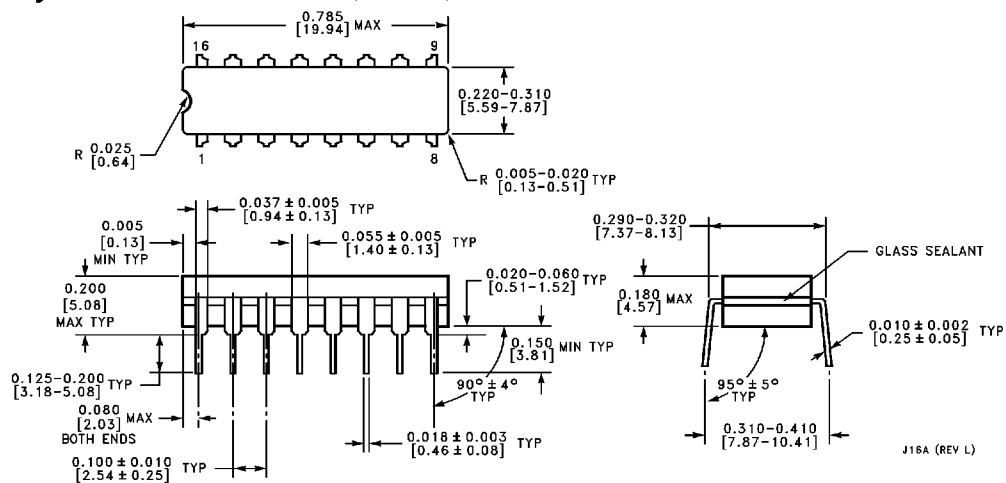
16-Lead Ceramic Dual-In-Line Package (J) Order Number 5442ADMQB or DM5442AJ NS Package Number J16A
