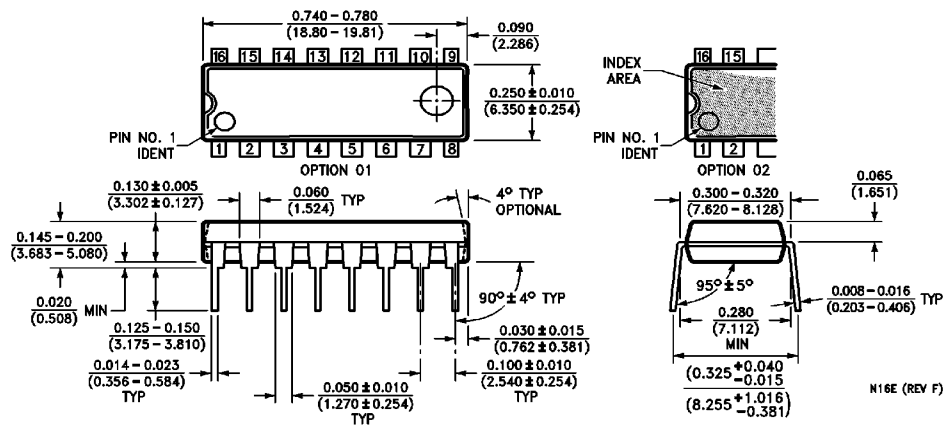
16-Lead Molded Dual-In-Line Package (N) Order Number DM7442AN NS Package Number N16E
