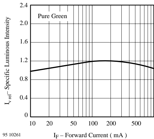
Figure 27. Specific Luminous Intensity vs. Forward Current
