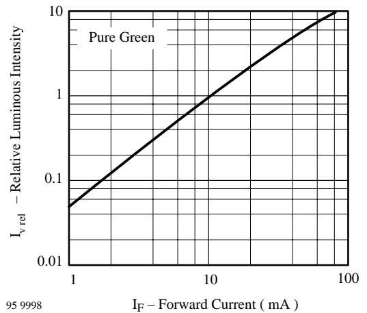
Figure 28. Relative Luminous Intensity vs. Forward Current
