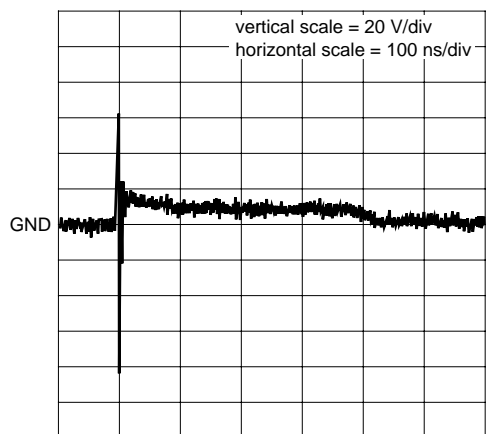
Fig 16. PESD5Z7.0: Clamped +8 kV ESD pulse waveform (IEC 61000-4-2 network)
