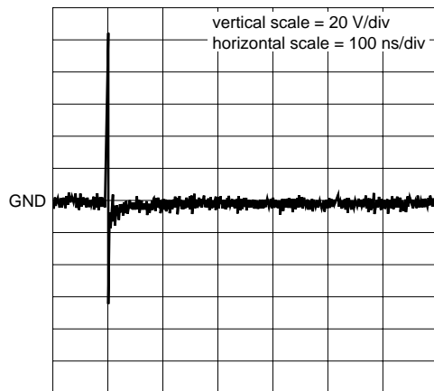
Fig 15. PESD5Z6.0: Clamped -8 kV ESD pulse waveform (IEC 61000-4-2 network)
