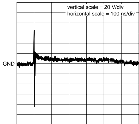
Fig 14. PESD5Z6.0: Clamped +8 kV ESD pulse waveform (IEC 61000-4-2 network)
