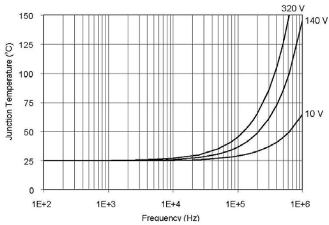
Figure 40. IRS2117/IRS2118 T_J vs. Frequency (IRFBC20) R_{GATE}=33\Omega , V_{CC}=15V
