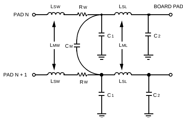
Figure 21. Package Parasitics
