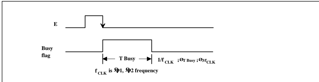
Figure 6 Busy Flag
