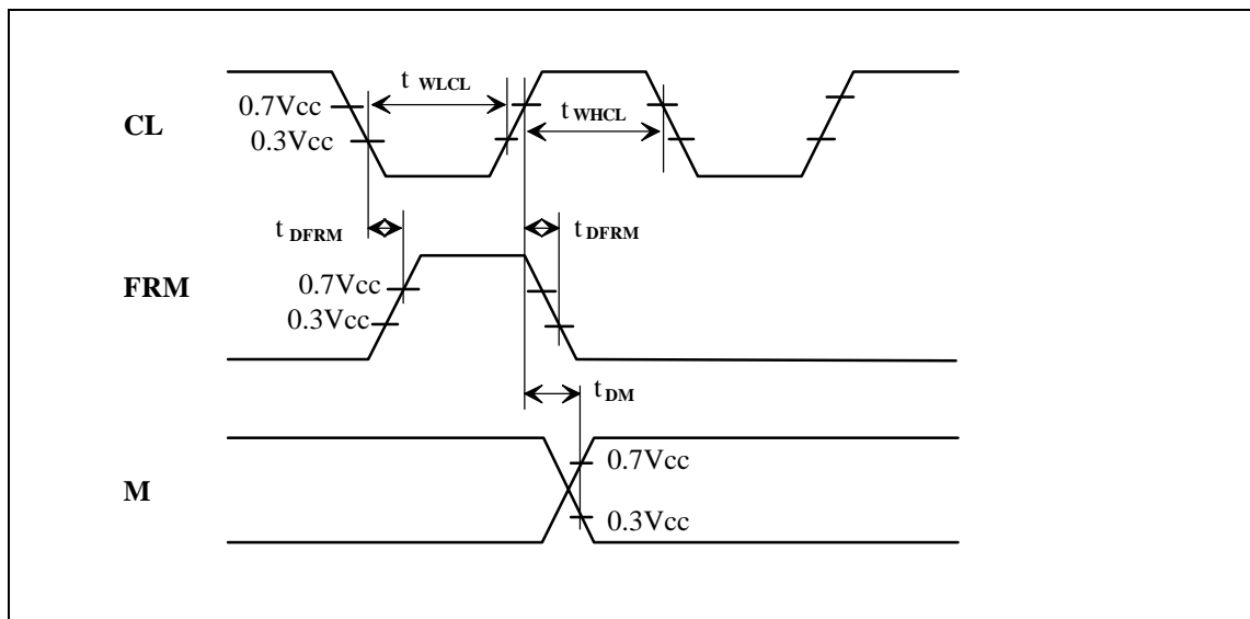
Figure 4 Display Control Signal Waveform
