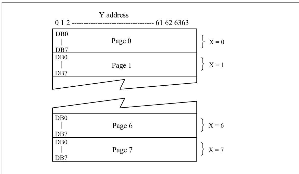
Figure 9 Address Configuration of Display Data RAM
