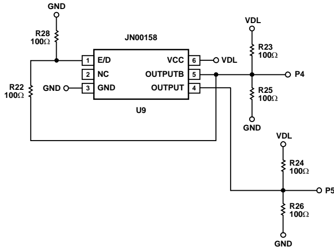
Figure 69. Evaluation Board Schematic—LVDS (continued)
