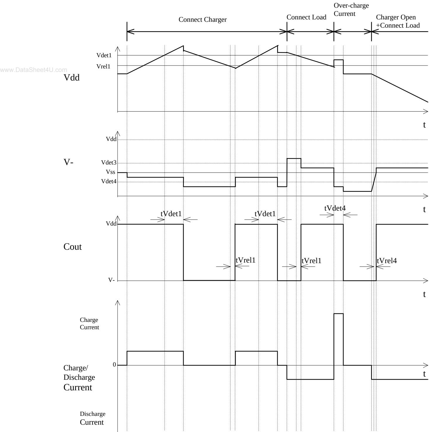
(1) Timing diagram of over-charge voltage and over-charge current
