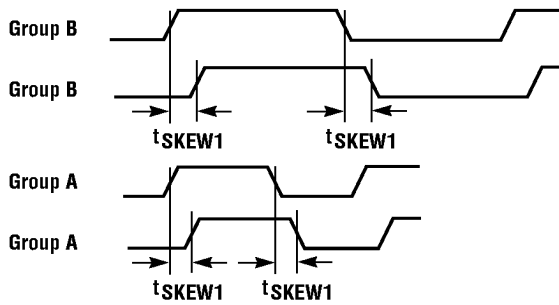
Figure 5. t_{SKEW1}
