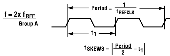
Figure 7. t_{SKEW3} (For Group B Feedback)
