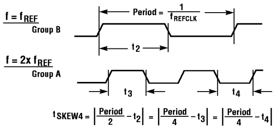
Figure 8. t_{SKEW4}
