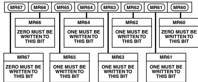
Figure 29. Mode Register 6
