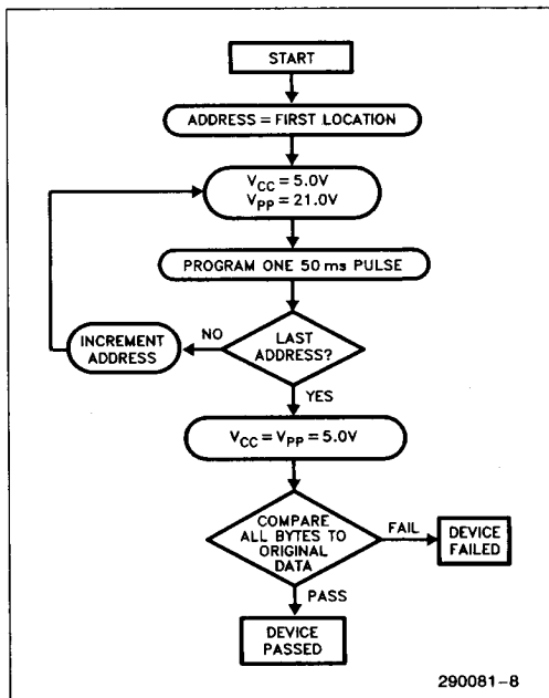
Figure 3. Standard Programming Flowchart
