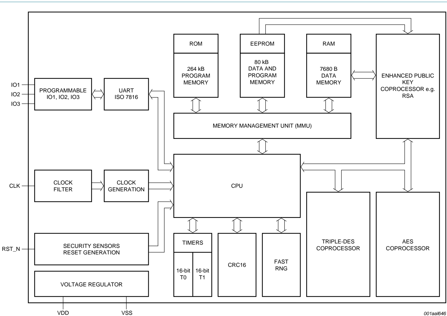
Fig 1. Block diagram
