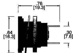
MFS470B-WP WATERTIGHT
