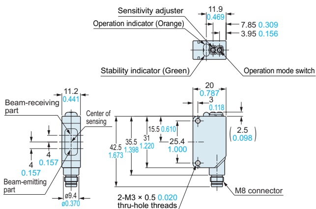
CX-49□-Z CX-48□-Z CX-42□-Z Sensor
