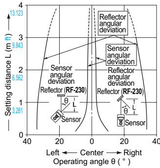
CX-481□ Retroreflective type
