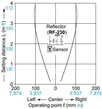
CX-481□ Retroreflective type
