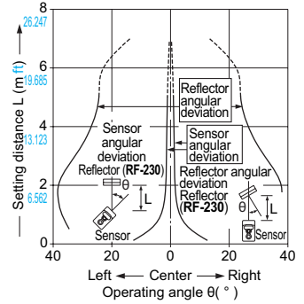
CX-482□ Retroreflective type
