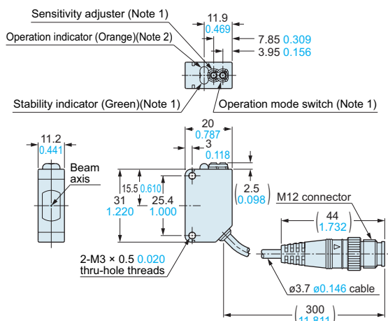
CX-41□-J Sensor
