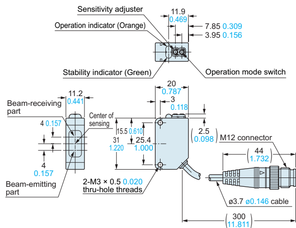
CX-49□-J CX-48□-J CX-42□-J Sensor
