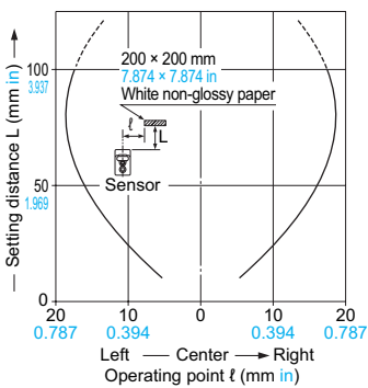
CX-421□ Diffuse reflective type
