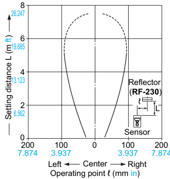
CX-482□ Retroreflective type
