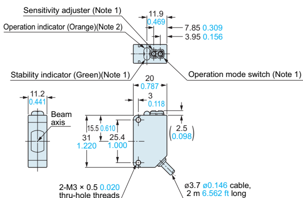
CX-41□ Sensor
