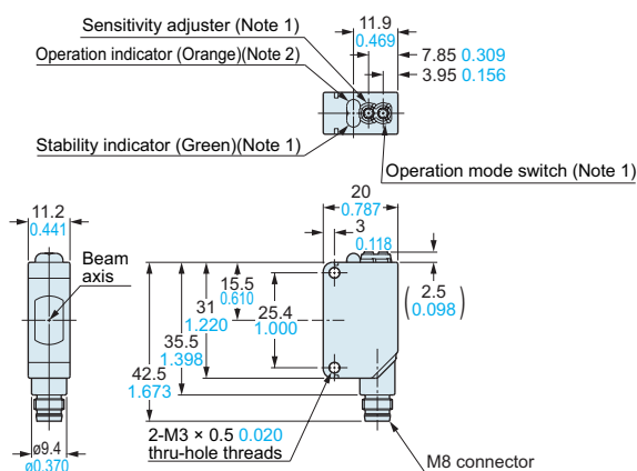
CX-41□-Z Sensor
