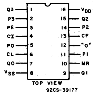
TERMINAL ASSIGNMENT
