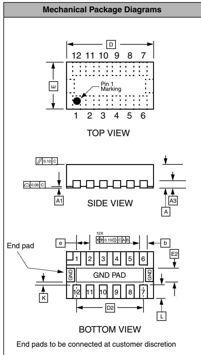
Dimensions for 12-Lead, 0.4mm pitch NuDFN package
