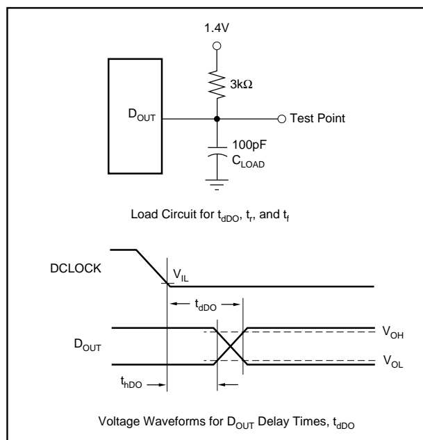
FIGURE 3. The Timing Relationship Between DCLOCK and the Serial Data Output at DOUT of the Converters is Shown Here. V_{IL} and V_{OL} is defined at 10% above logic low, V_{OH} is defined at 10% below logic high.
