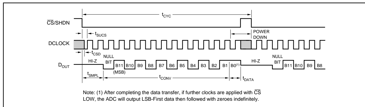
FIGURE 2. The Standard Timing Diagram for the ADS7816, ADS7817, and ADS7822 is Shown Here. In this figure \overline{CS} and the transfer of the DOUT to the processor is initiated by the falling edge of DCLOCK.
