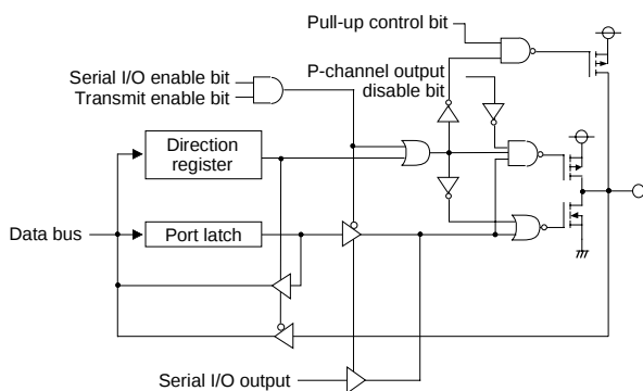
Fig. 19 Port block diagram of 3804 group (1)
