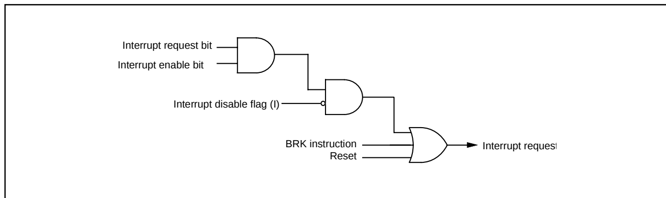
Fig. 26 Interrupt control
