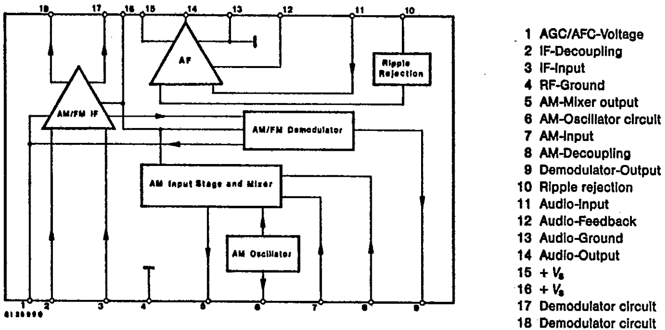
Fig. 1 Block diagram and pin connections
