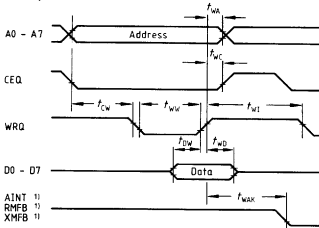
Figure 3 μP Write Timing
