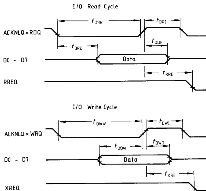
Figure 4 DMA Timing
