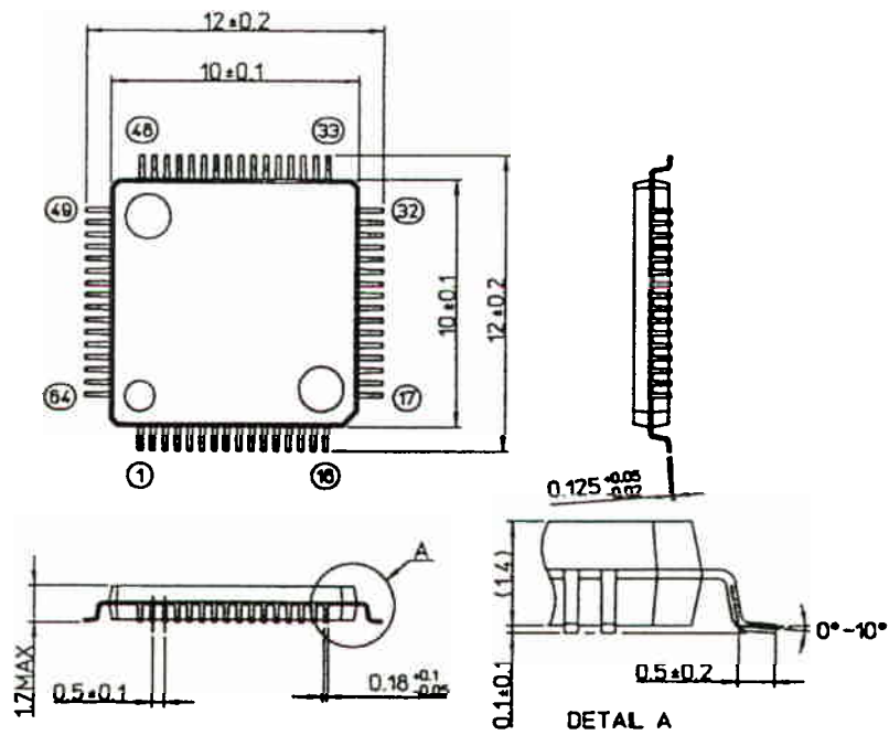
Figure 8 Package Information
