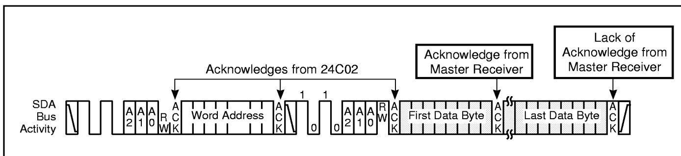
Figure 9. Sequential Read
