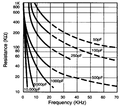
Resistance vs Oscillator Frequency – ET15
