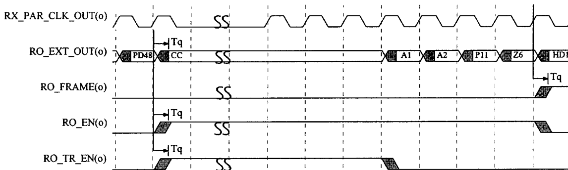
Figure 19. Receive External Timing with RO_TR_EN
