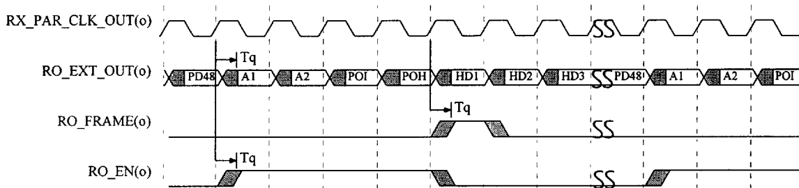
Figure 18. Receive External Timing
