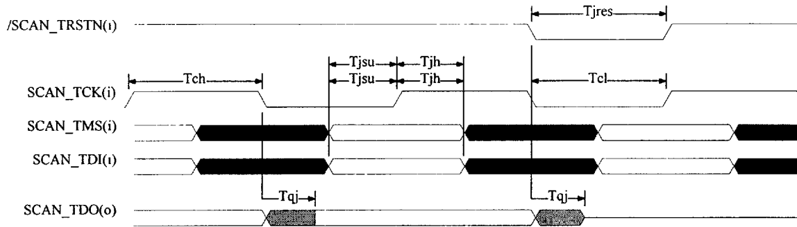
Figure 26. JTAG Timing
