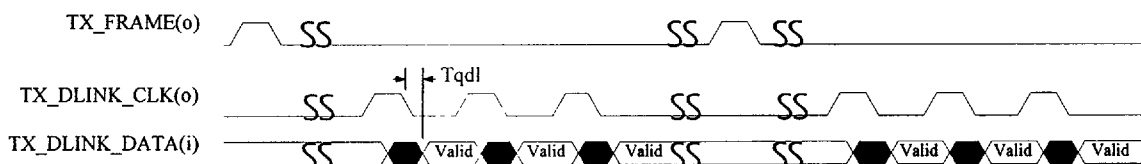
Figure 13. Transmit Data Link Channel Timing
