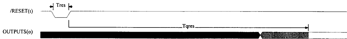
Figure 24. Reset Timing
