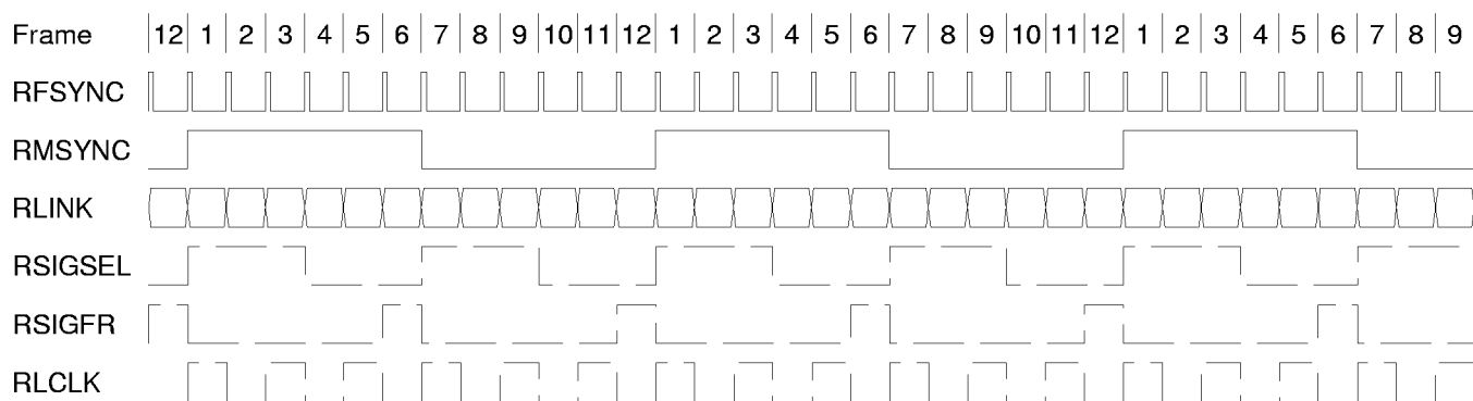
Figure 18. T1DM Multiframe Receive Timing
