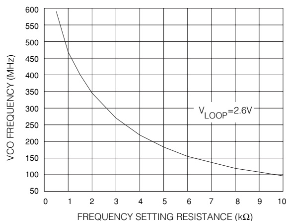
Fig. 12 VCO Frequency
