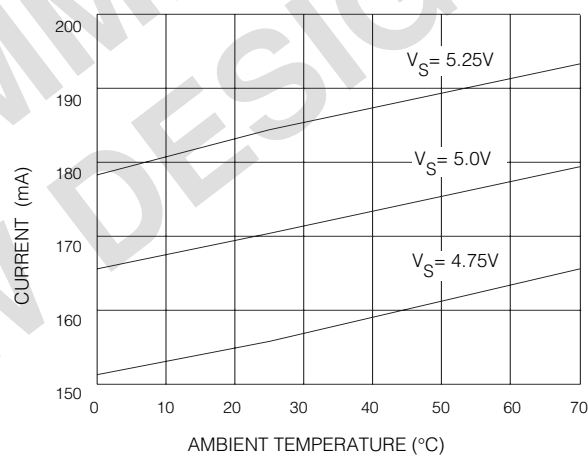
Fig. 15 Supply Current
