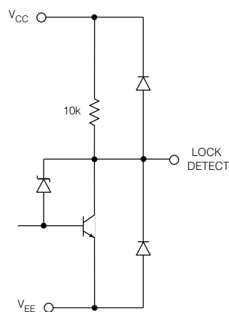
Fig. 5 Pin No. 20 Lock Detect
