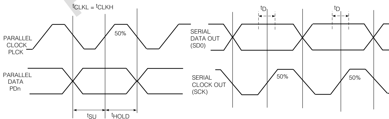
Fig. 9 Waveforms
