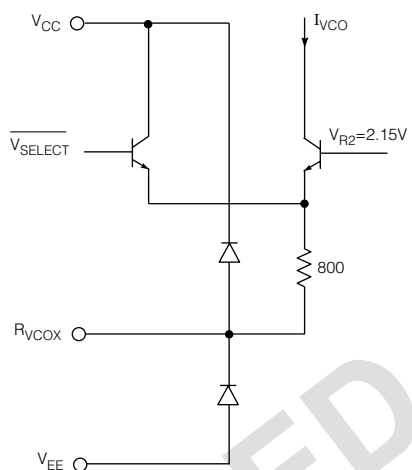
Fig. 7 Pins No. 31 - 34 Frequency Setting Registers R_{VCO0} - R_{VCO3}
