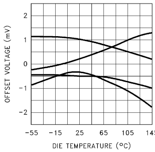
Offset Voltage vs Die Temperature (4 Samples)
